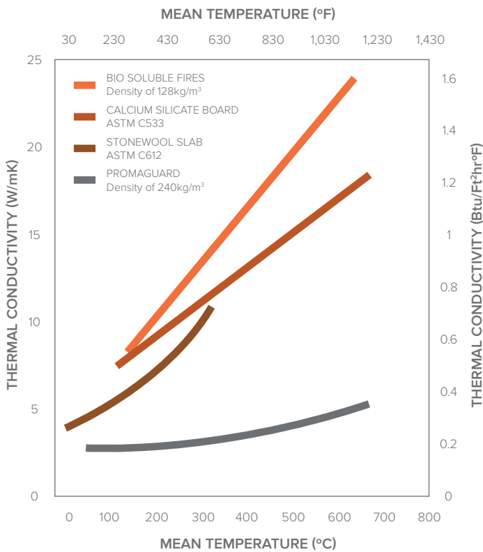
Third-party tests show how layers of Promaguard suppress thermal conductivity and delay the onset of a fire
